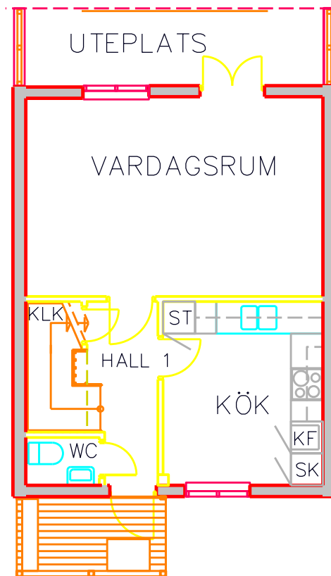
Bottenplan
