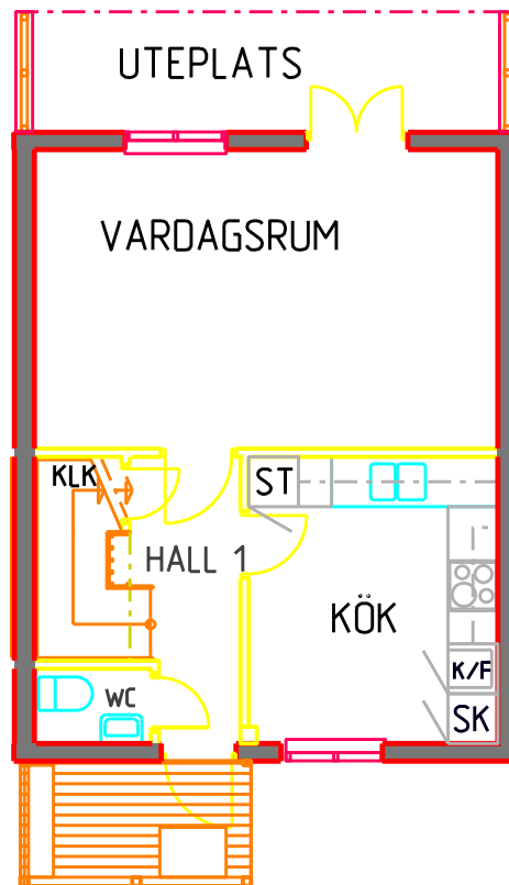
Markplan
