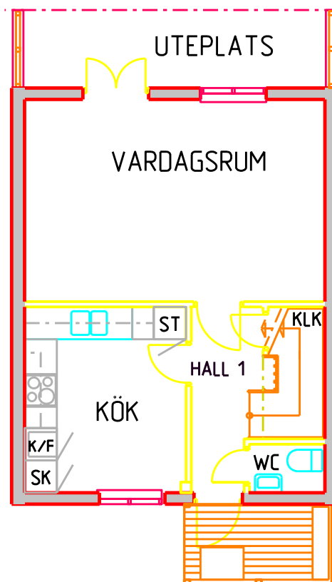
Bottenplan
