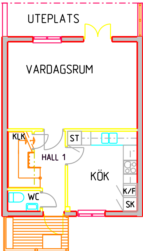
Bottenplan
